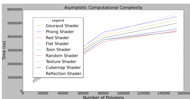
Figure 14: Rendering process: curves comparison
