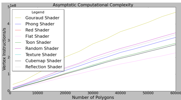
Figure 12: Vertex shader: curves comparison
