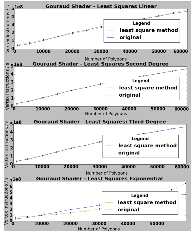
Figure 10: Automatic Adjustments: vertex shader
