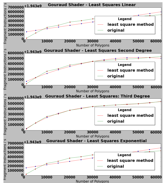
Figure 11: Automatic Adjustments: fragment shader
