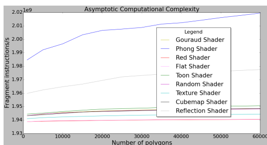
Figure 13: Fragment shader: curves comparison
