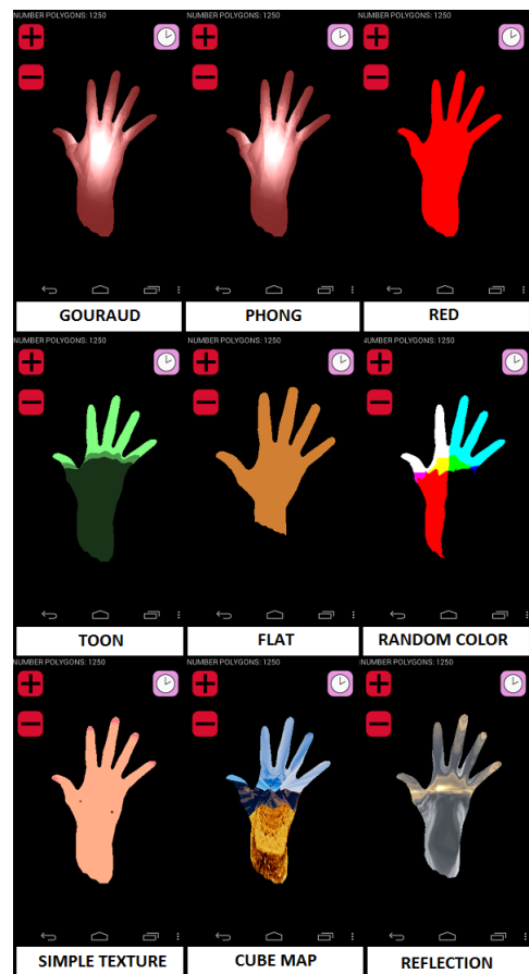
Figure 5: Implemented Shaders
